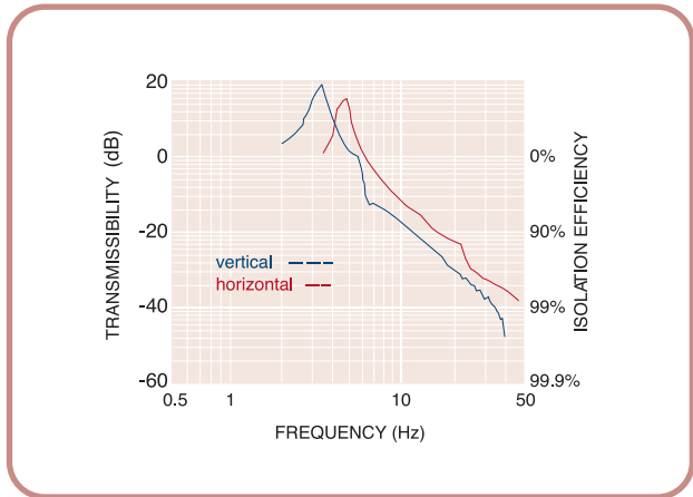
Vertical and Horizontal Transmissibility of Thorlabs' Passive Vibration Isolators.
