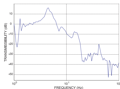
Vertical Transmissibility of Passive Isolation
