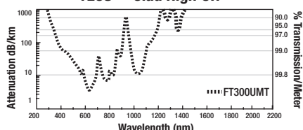
TECS™ Clad High OH
